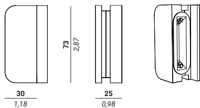
Dimensioni contropiastra / Dimensions counterplate
