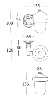
7012 PORTA-ROTOLO PAPER ROLL HOLDER
