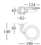
7205 PORTA-SAPONE SOAP DISH HOLDER
