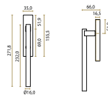
tilt-and-turn system
