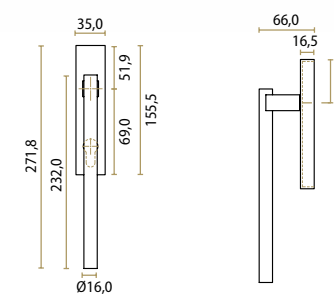
tilt-and-turn system
