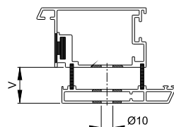
Aluminium-Profil
