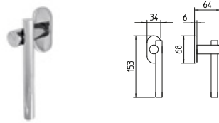
1672/DK MARTELLINA DK drehkipp system
