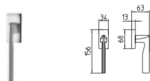
1462/DK MARTELLINA DK drehkipp system
