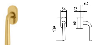
S62/DK MARTELLINA DK drehkipp system
