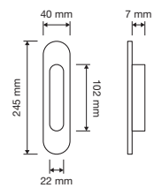
Liberty | 1273 CI 1972 OF (Ø int. 16 mm)
